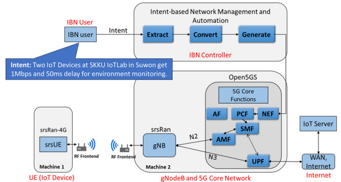
Fig. 1. Architecture of the 5G Core Network with Intent-Based Network Management and Automation
